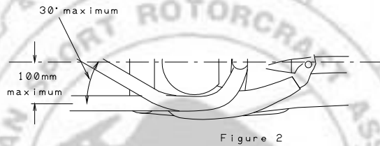
Range of Angles of Sholder Straps
